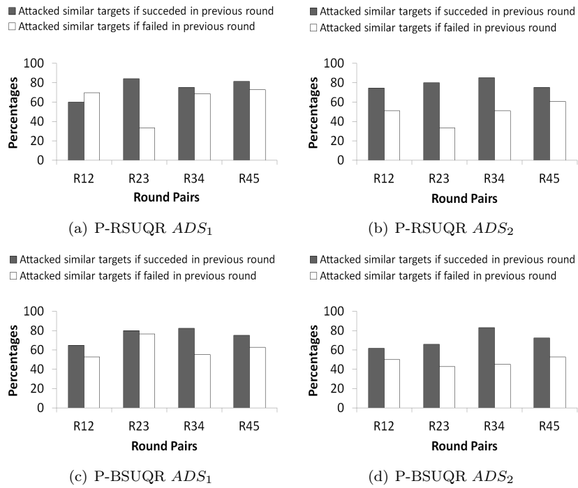
Figure 2: Evidence for adaptivity of attackers
