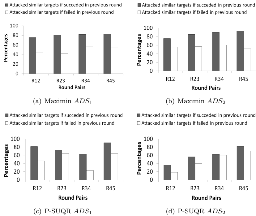
Figure 1: Evidence for adaptivity of attackers
